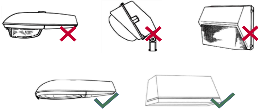
Figure 49: No Uplight Luminaires
